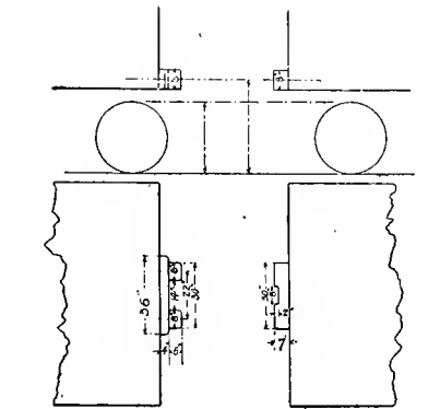
Figs. 5548-5549. THE LOCATION OF BUFFER-BLOCKS AND BUFFER-BEAM.
